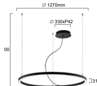
LED 61W 120° - 3000K - 4100lm code : V4224200 Black
