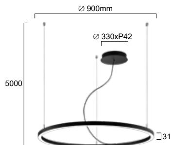
LED 48W 120° - 3000K - 3200lm code : V4224100 Black
